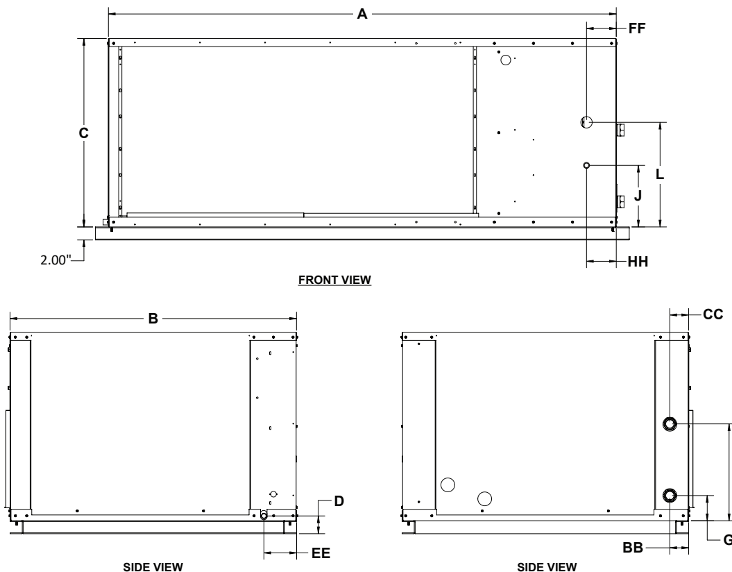
Figure 15: WSLH Unit Dimensions
